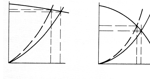
FIG. 16 – EFFECT OF FAN CURVE SLOPE
