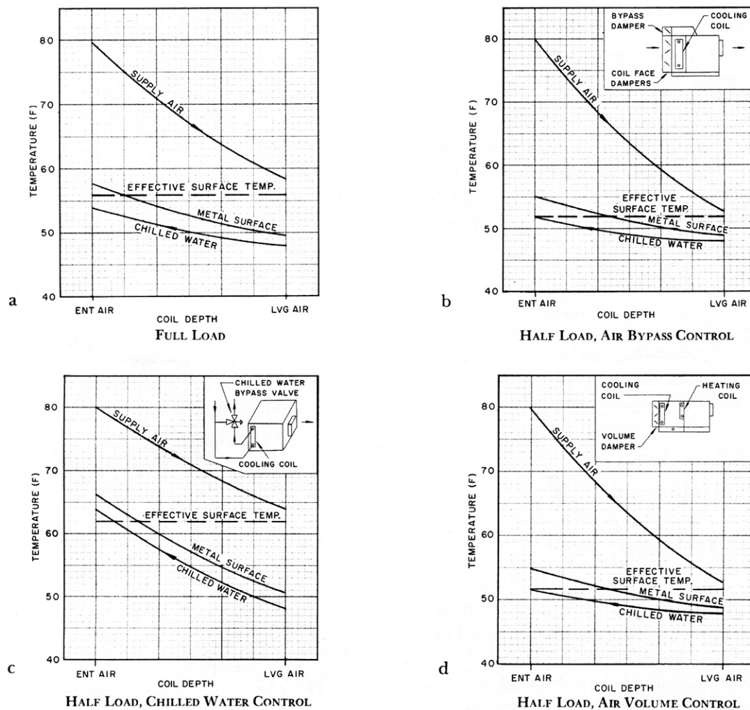
FIG. 35 — TYPICAL COOLING COIL PROCESSES
