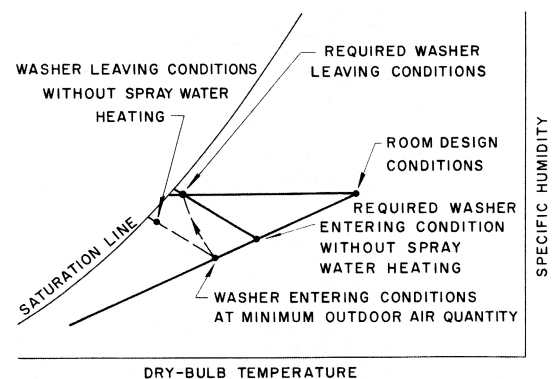
FIG. 45 — EFFECT OF SPRAY WATER HEATER
