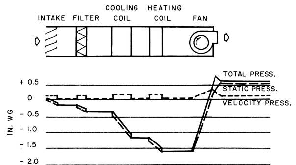
FIG. 30 — PRESSURE VARIATIONS (DRAW-THRU UNIT)
