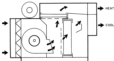
FIG. 29 — AIR FLOW — MULTI-ZONE UNIT
