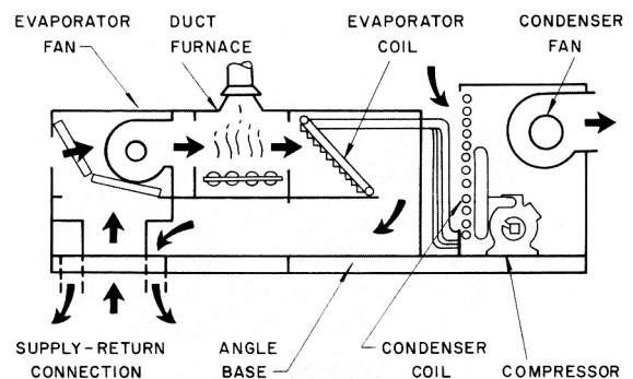
FIG. 51 — SELF-CONTAINED UNIT
