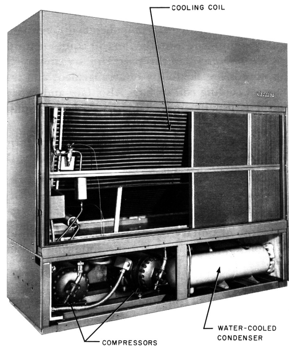
FIG. 50 — SELF-CONTAINED UNIT
