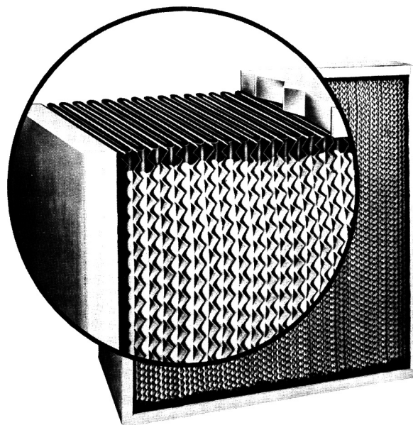
FIG. 59 — HIGH EFFICIENCY DRY FILTER
