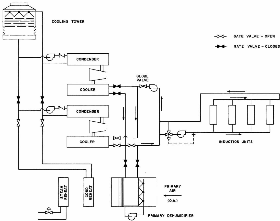
Fig. 11 – Off-Season Cooling Using a Heat Pump System
