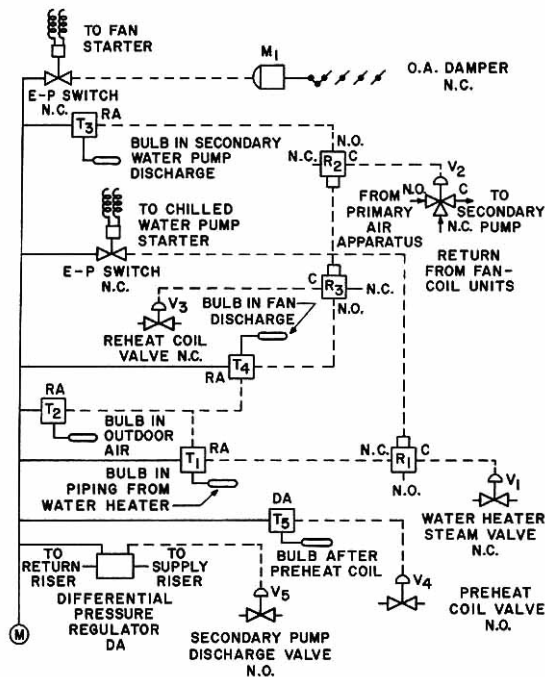
Fig. 20 – Typical Control Diagram Pneumatic
