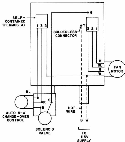
Fig. 21 - Control Package, Fan-Coil Unit, Manual Three-Speed Fan Control With Automatic On-Off Waterflow
