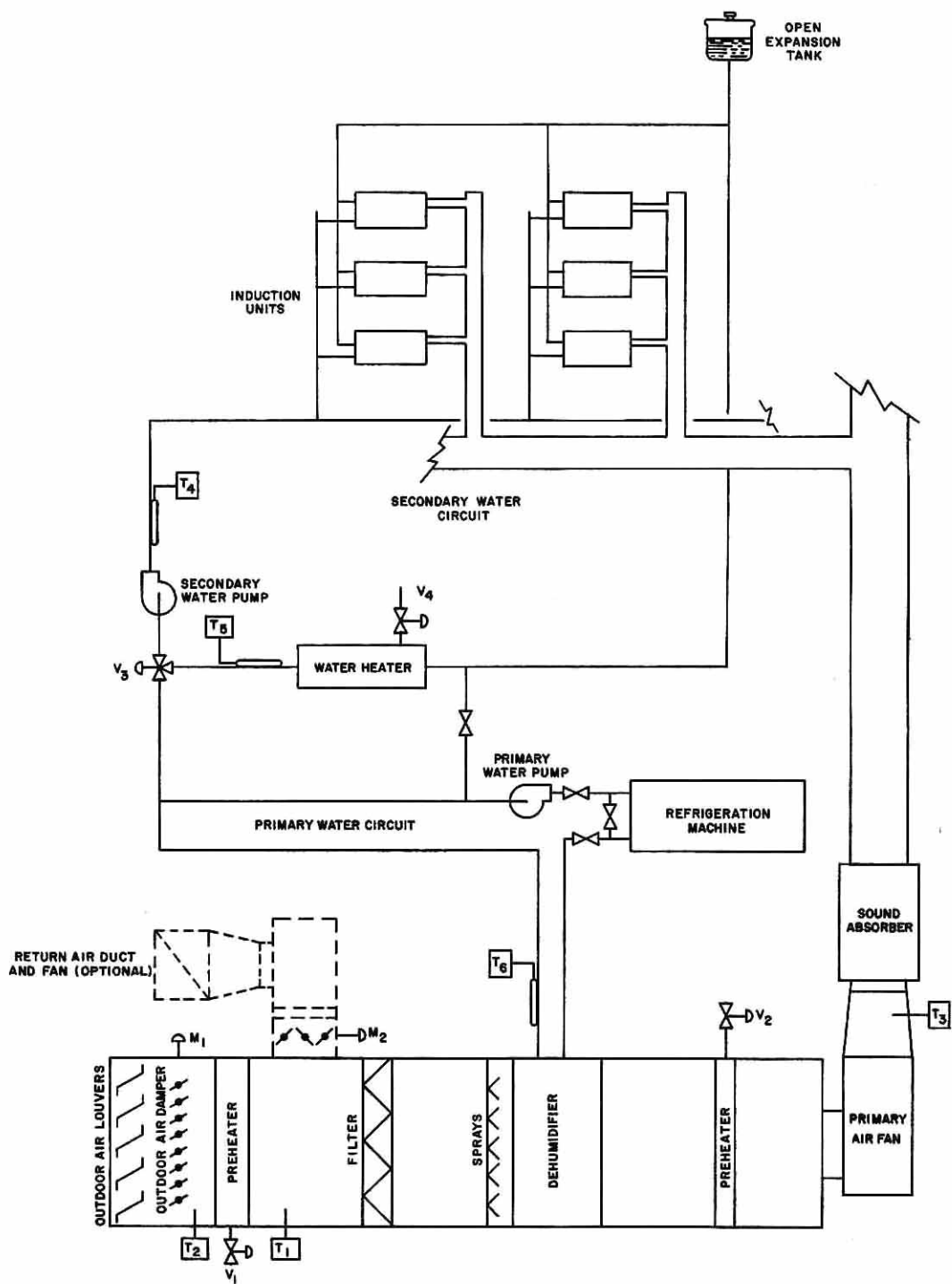
Fig. 1 – Typical Induction Unit System
