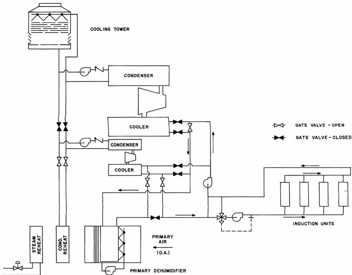
Fig. 12 – Off-Season Cooling With Auxiliary Cooling In Parallel
