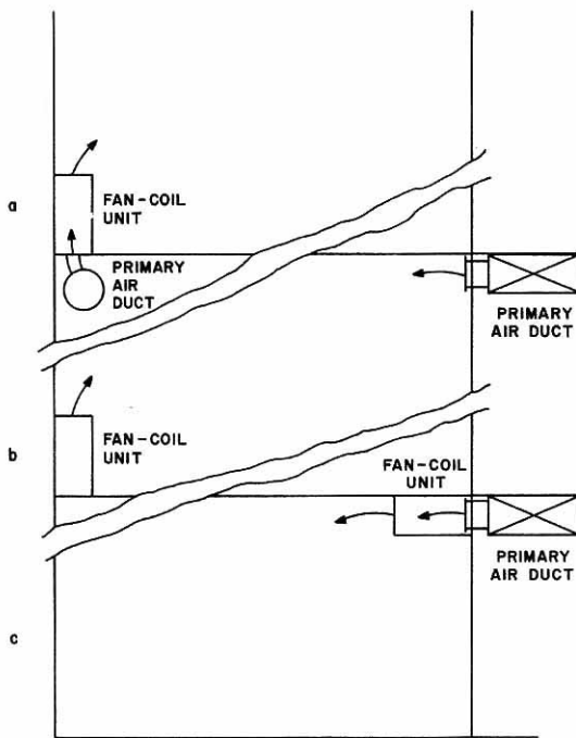
Fig. 16 – Primary Air Fan-Coil Arrangements
