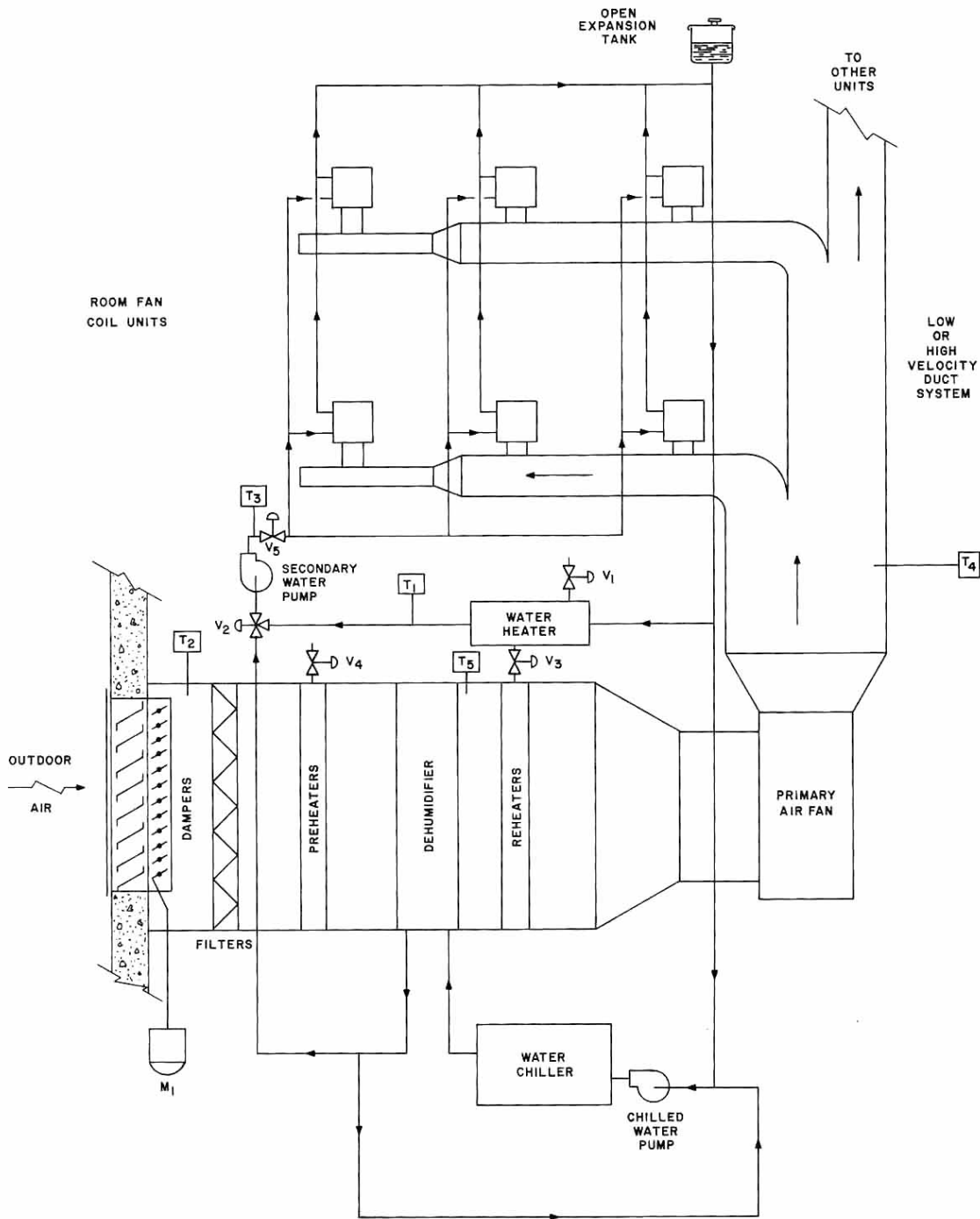
Fig. 17 – Primary Air Fan-Coil System
