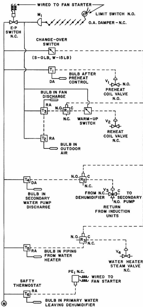
Fig. 8 – Induction Unit System Control
