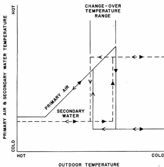
Fig. 15 – Temperature Schedule
