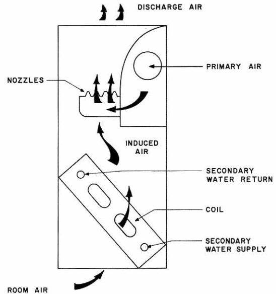
Fig. 2 – Typical Induction Unit
