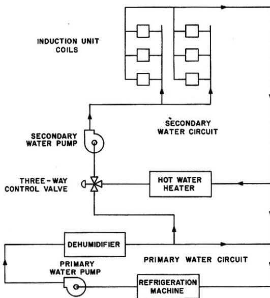
Fig. 7 – Water Distribution System
