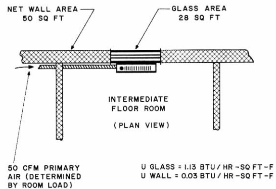
Fig. 2 – Typical Induction Unit
