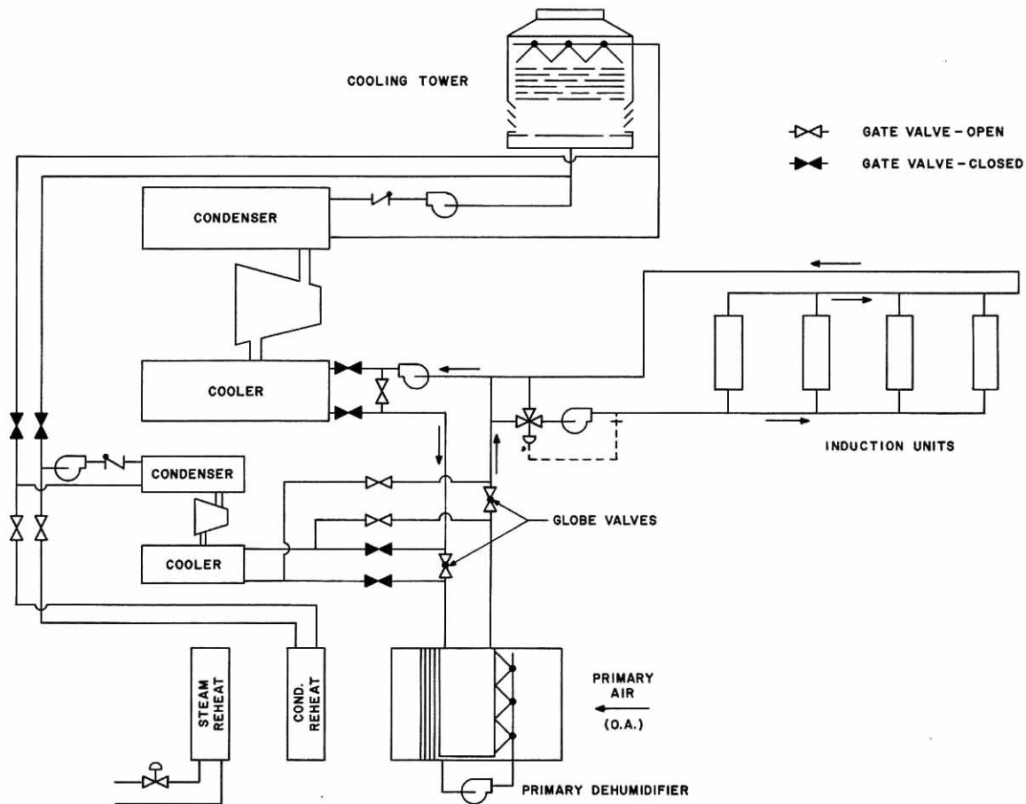
Fig. 13 – Off-Season Cooling With Auxiliary Cooling In Series
