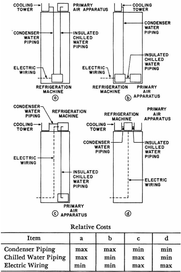
Fig. 4 – Relative Location And Costs of Pipe and Wiring
